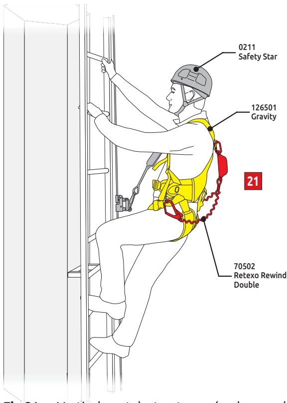
Fig.21 - Vertical metal structures (such as cableway pylons and wind farm turbine poles) are often equipped with ladders for progression combined with a vertical anchoring cable on which fall arrest devices can be installed. These devices are designed to follow the operator during movement and intervene to arrest any fall.
